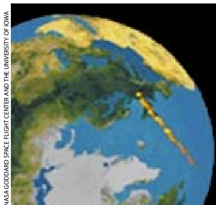
ULTRAVIOLET STREAK, superimposed on the visible earth, may be the wreckage of a small comet.
