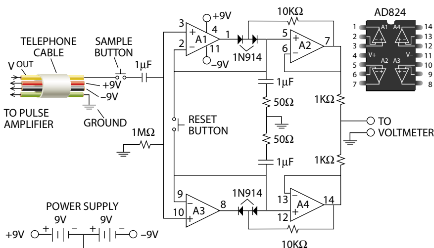
DUAL PEAK DETECTOR allows measurement with a handheld digital voltmeter.
