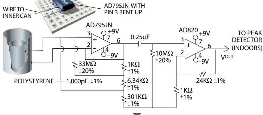
PULSE AMPLIFIER puts out a voltage spike when a drop passes through.
